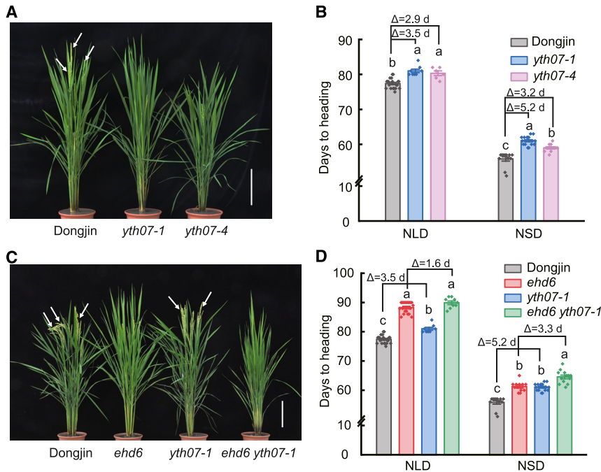
Figure 3. YTH07 participates in promoting rice flowering.
